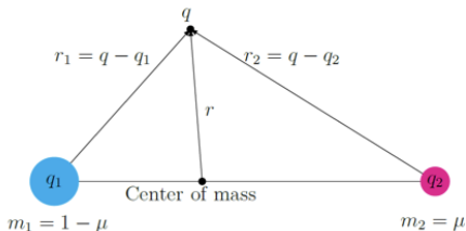
The three-body constraint problem
